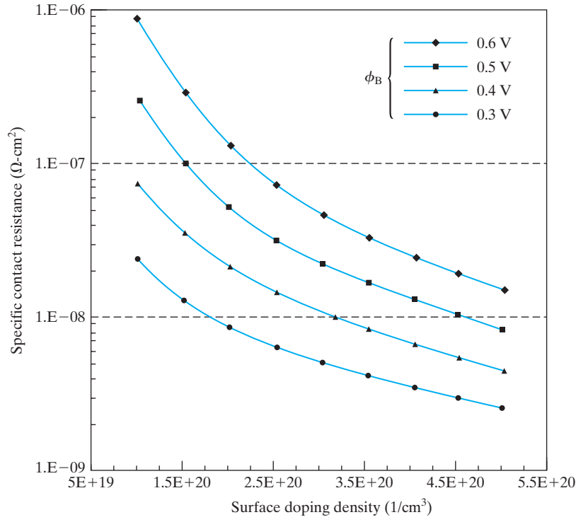
FIGURE 4-46 Theoretical specific contact resistance. (After [12].)
